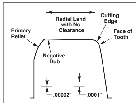
Conventional tooth profile as measured and graphed by our electronic gaging equipment
