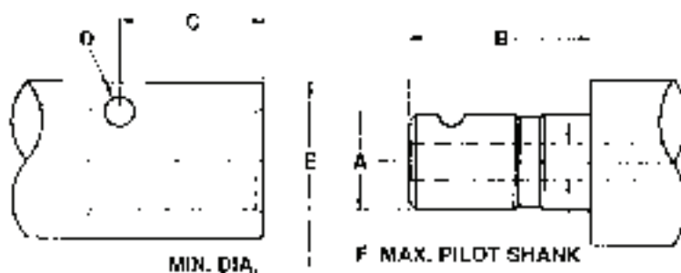
Pin Drive
