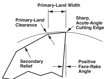
Only the sharp cutting edge is in contact with the workpiece.
