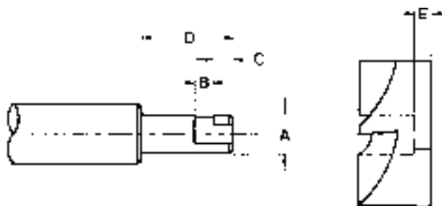
Inverted Drive
