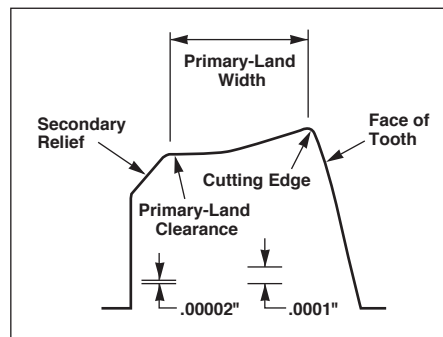
METCUT tooth profile as measured and graphed by our electronic gaging equipment
