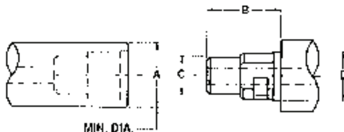
Radial Drive
